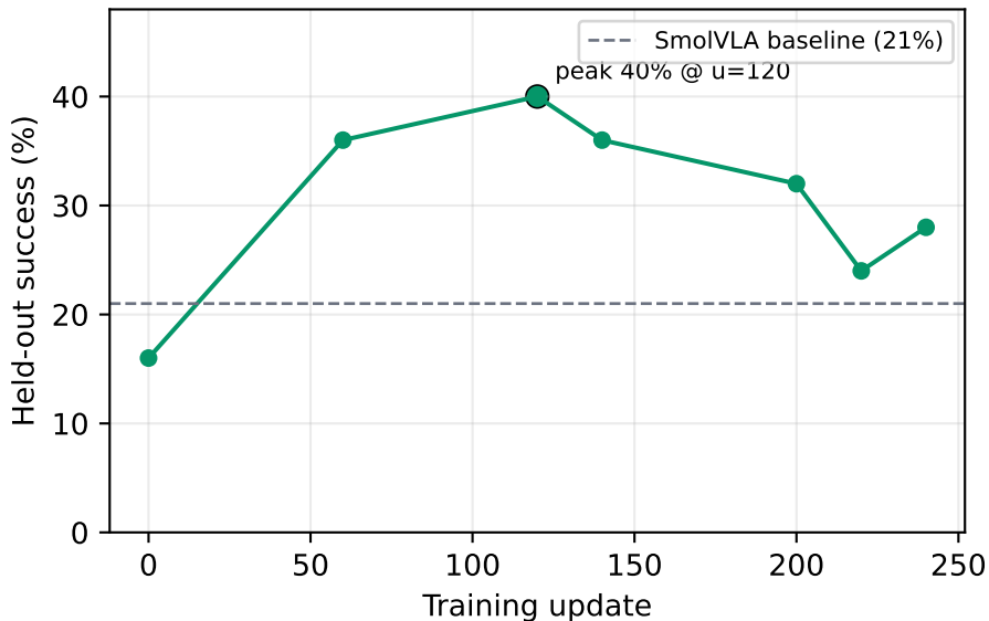
Direct sparse PPO: selected 25-episode checkpoints
