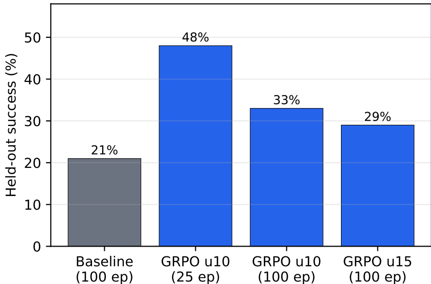
Short vs long held-out evaluation (same policy family)
