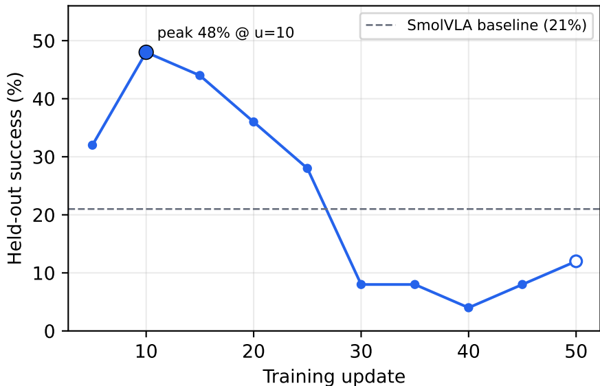
Environment-reward GRPO (group 8): 25-episode held-out sweep
