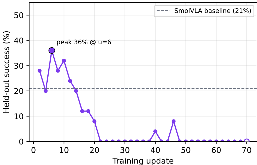
World-model-reward GRPO: held-out push-v3 success vs update
