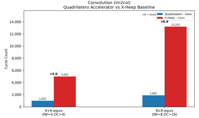
Fig. 5. Cycle counts for convolution (im2col) on Quadrilatero vs. scalar X-HEEP for two small input configurations.
