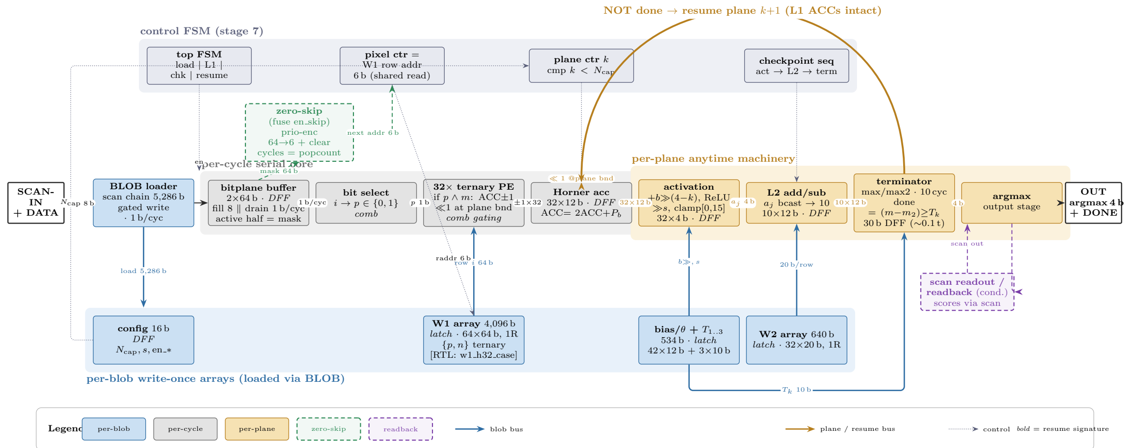
Figure 1: Chrome Chain v1 logical datapath ( 64 \rightarrow 32 \rightarrow 10 ternary MLP, bit-serial, plane-major). Three timing domains: blue = per-blob write-once arrays (loaded once per model swap), grey = per-cycle serial core (pixel/MAC cadence), amber = per-plane anytime machinery (checkpoint cadence). The bold amber return path ( not done → resume plane k+1 ) is the architectural signature. Dashed green = fuseable zero-skip; dashed purple = conditional scan readback. Every edge carries its bus width; every block names its storage type. Stage-2 (W1) structure is extracted from the RTL; all other blocks are annotated from the v1 spec (Fig. 1, Tables 1–2) and have no RTL yet.
