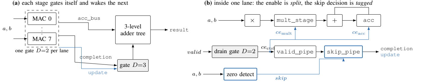
Fig. 1. Architecture. (a) The array and the adder tree each own an independent completion-aware gate sized to their own pipeline depth D ; there is no central controller, and the update bus (blue) is the only wire the sparsity extension adds between stages. (b) Within a lane the clock enable is split. ce_{ctrl} is triggered by the raw valid and is never masked, so the drain counter is structurally blind to sparsity; ce_{mult} and ce_{acc} additionally carry the skip term and gate only the two wide register banks, which hold 64 of the lane's \approx 70 flip-flops. The skip decision is registered as skip_p alongside valid_p , so the accumulate stage consults the tag belonging to its own item rather than the current input bus.
