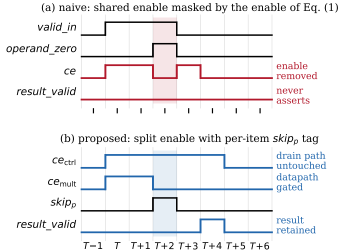
Fig. 2. The composability hazard. A zero operand at T+2 lands inside the drain window of the item that entered at T+1 . (a) Masking the shared enable strands that item; because the drain counter runs regardless, the window closes and the result is never produced. (b) Splitting the enable leaves the drain path untouched and gates only the datapath, so the result is retained.
