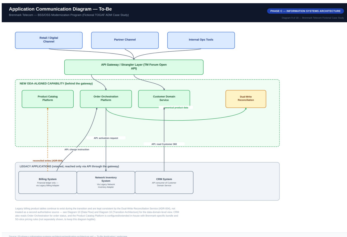
Diagram 9 — Application Communication Diagram, To-Be
