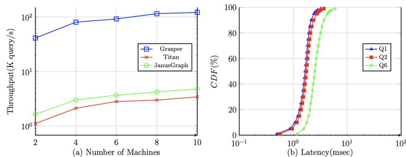
Figure 14: [Best viewed in color] (a) Throughput on AMiner for {Q1, Q2, Q6}; (b) CDFs of Grasper's query latency for {Q1, Q2, Q6} (using 10 machines)
