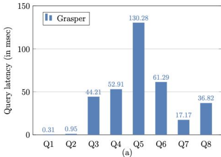
Figure 17: (a) Query latency (in msec ) of Q1-Q8 on Twitter by Grasper (using 10 machines); (b) Throughput of Grasper on Twitter for {Q1, Q2, Q6}
