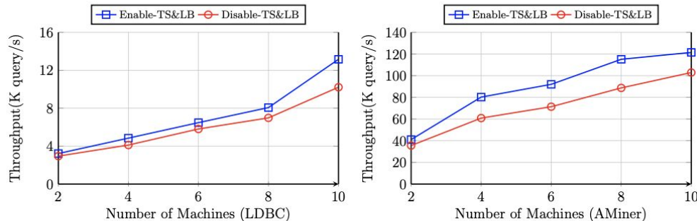
Figure 15: (a) Throughput of Grasper on LDBC for {IS1-IS4}, and (b) throughput of Grasper on AMiner for {Q1, Q2, Q6}, w/ and w/o TS&LB
