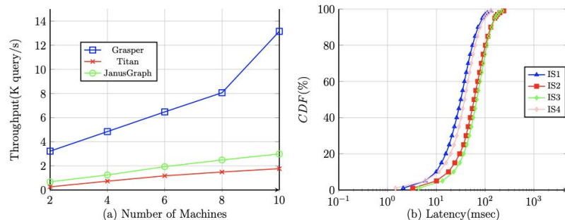
Figure 13: [Best viewed in color] (a) Throughput on LDBC for {IS1-IS4}; (b) CDFs of Grasper's query latency for {IS1-IS4} (using 10 machines)
