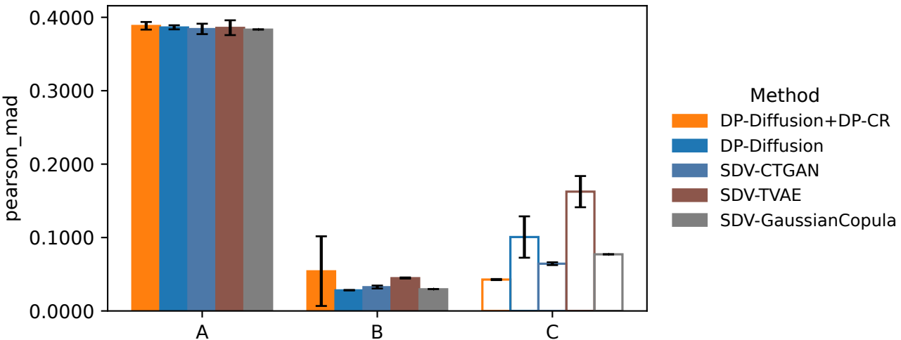
Pearson MAD (mean +/- std)
