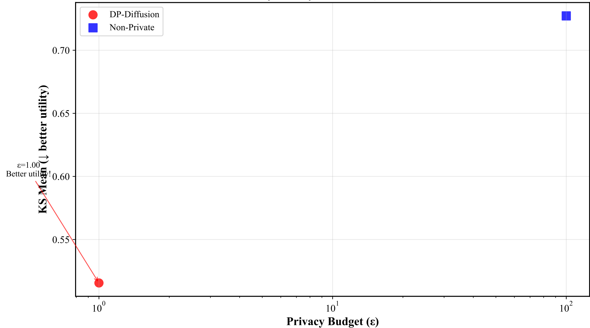
Privacy-Utility Tradeoff (Dataset B)
