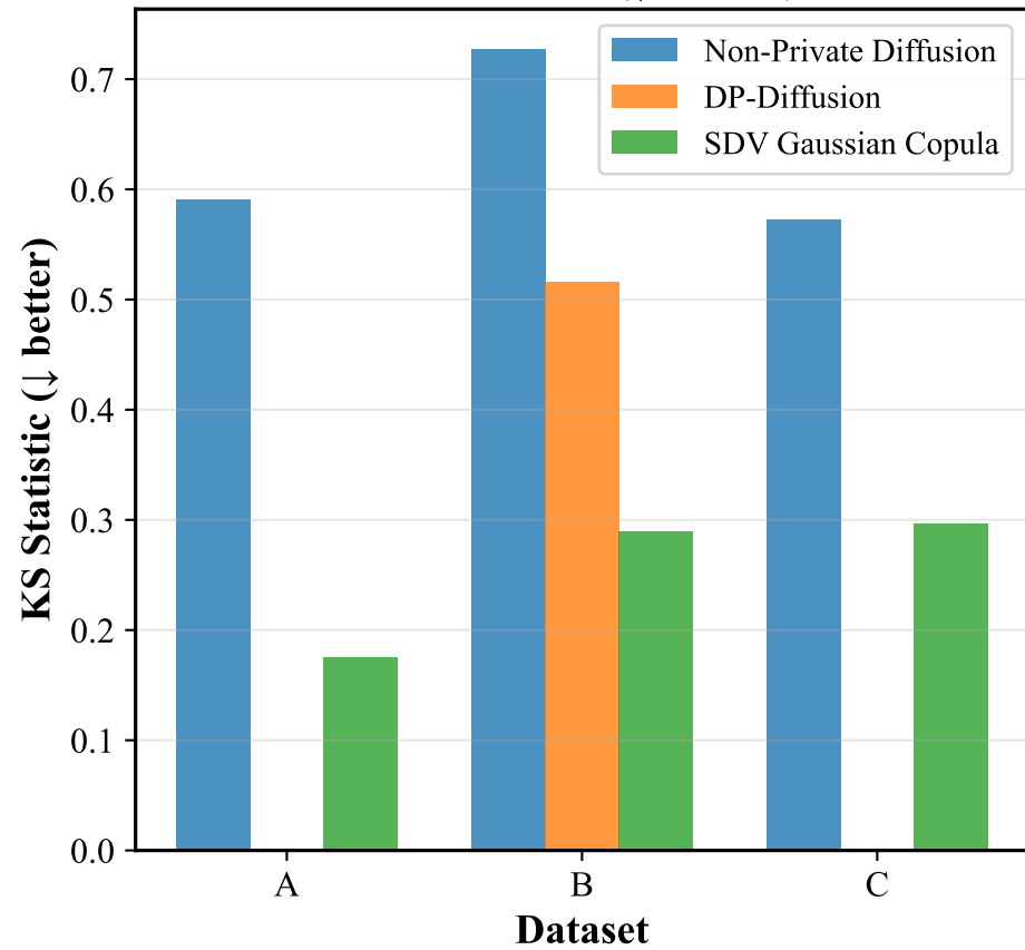
KS Statistic (↓ better)
