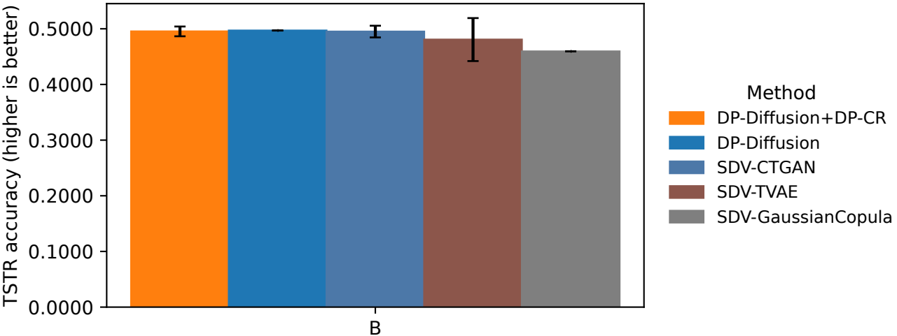
TSTR accuracy (mean +/- std)
