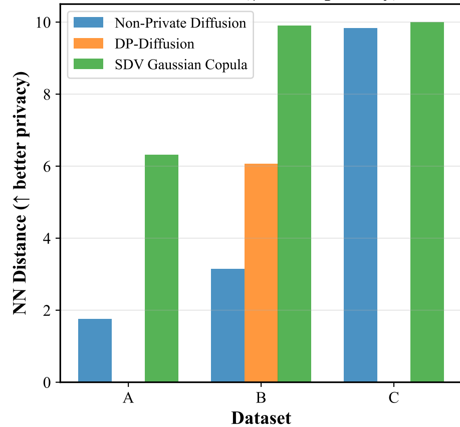
NN Distance (↑ better privacy)
