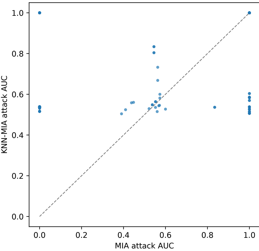
Privacy Agreement (n_both=288, n_exact=102)
