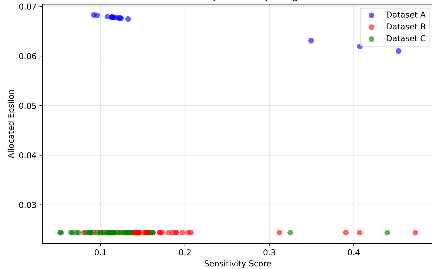
Privacy Level Distribution
