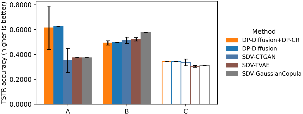
TSTR accuracy (mean \pm std)
