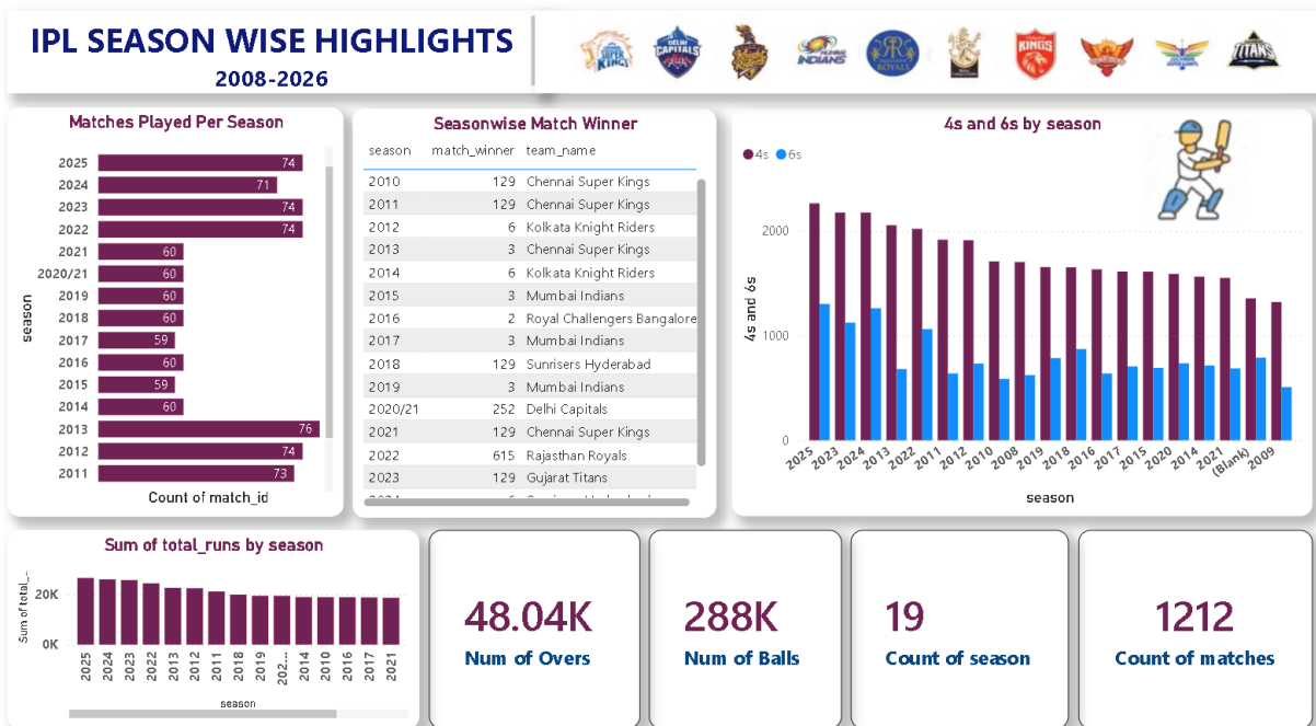
Figure 1: IPL Season Wise Analysis 2008-2026
