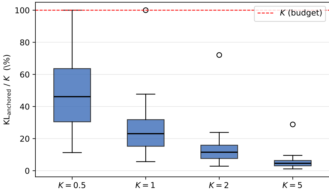
Budget utilization of anchored decoding
