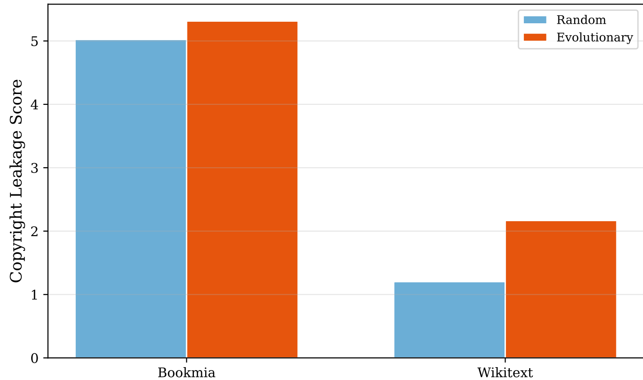
Dataset Comparison: BookMIA vs WikiText-103
