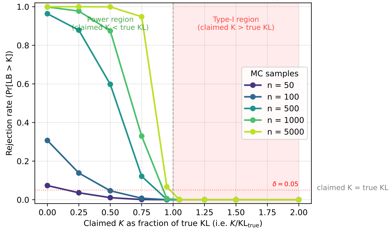
Auditor power & calibration (gpt2-medium vs gpt2)
