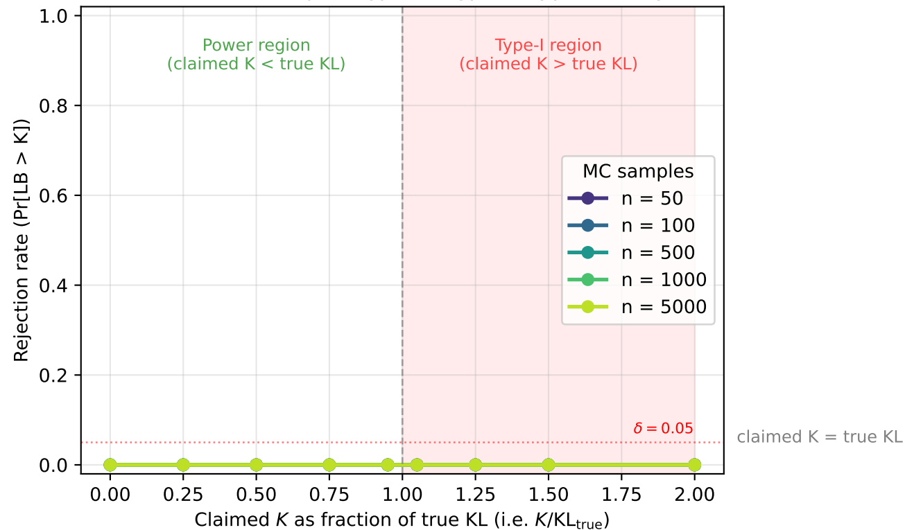
Auditor on null pair (gpt2 vs gpt2): Type-I sanity
