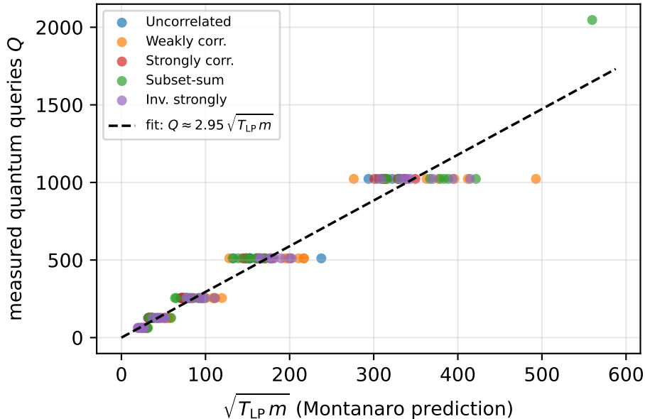
Measured quantum query count vs. Montanaro bound
