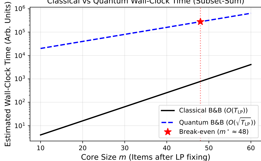
Classical vs Quantum Wall-Clock Time (Subset-Sum)
