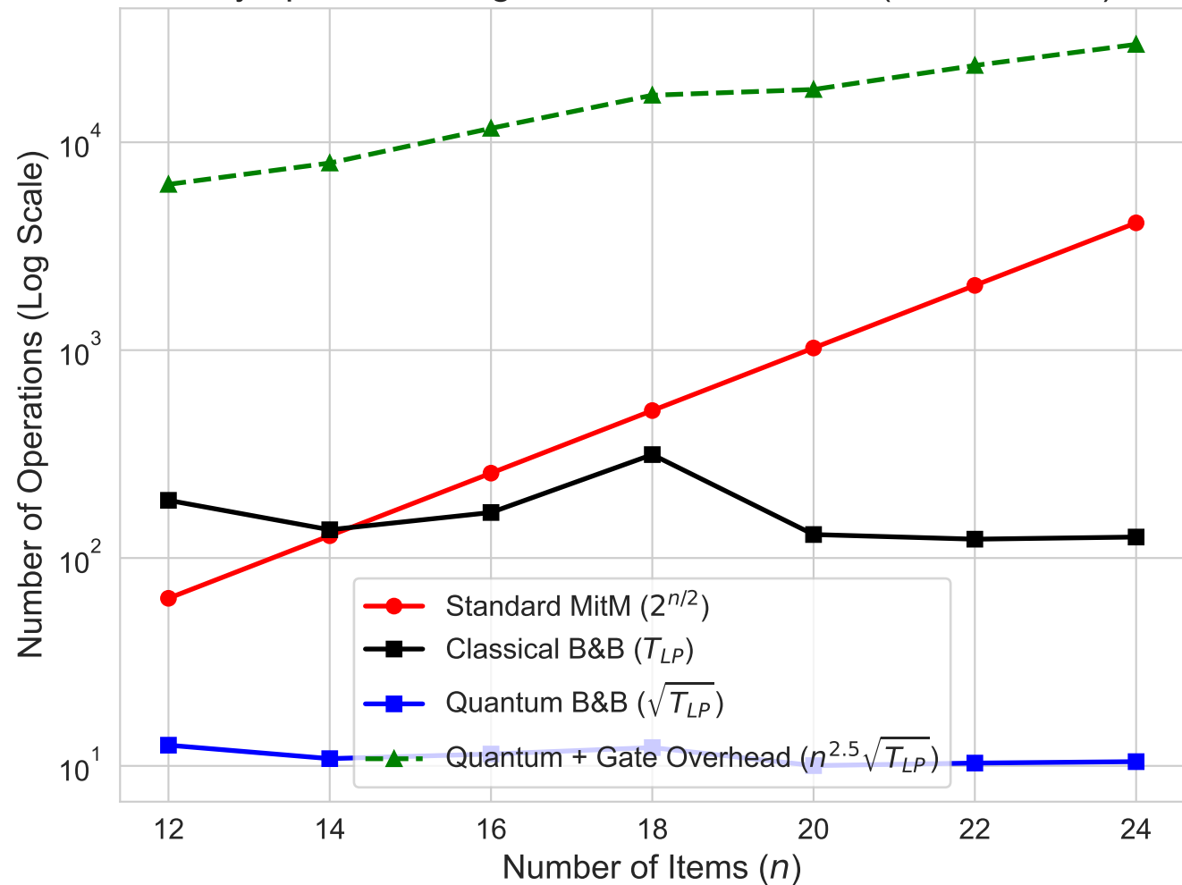
Asymptotic Scaling and Crossover Point (Subset-Sum)
