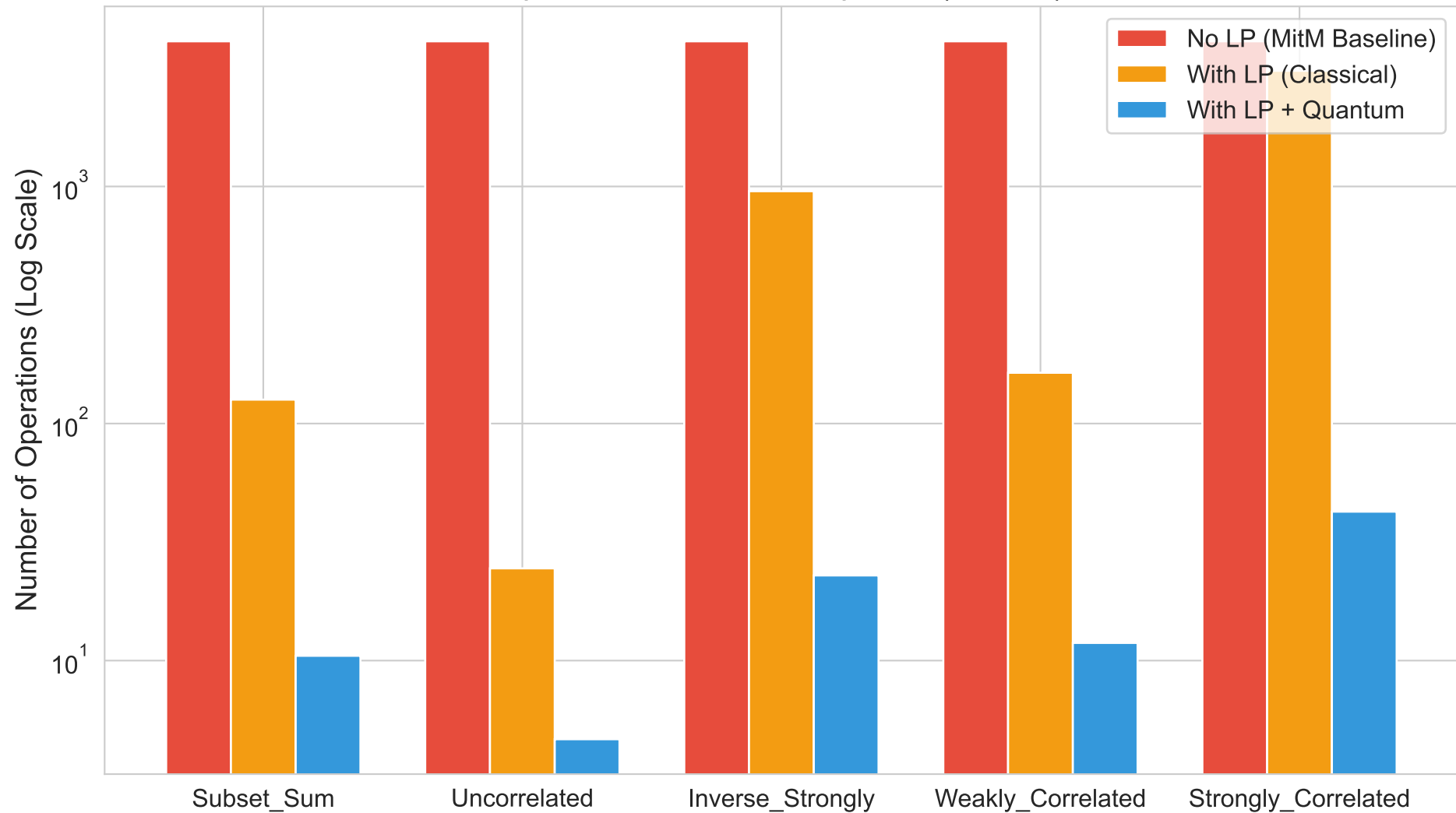
Operation Reduction Pipeline ( n = 24 )
