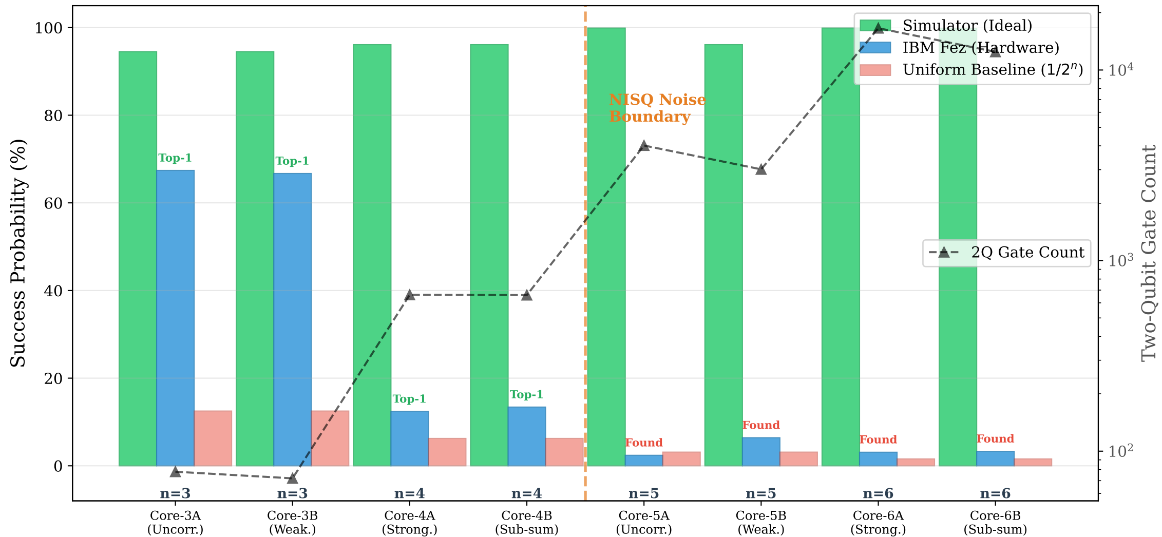
Quantum Hardware Validation: Simulator vs. IBM Fez ( n = 3 to n = 6 )
