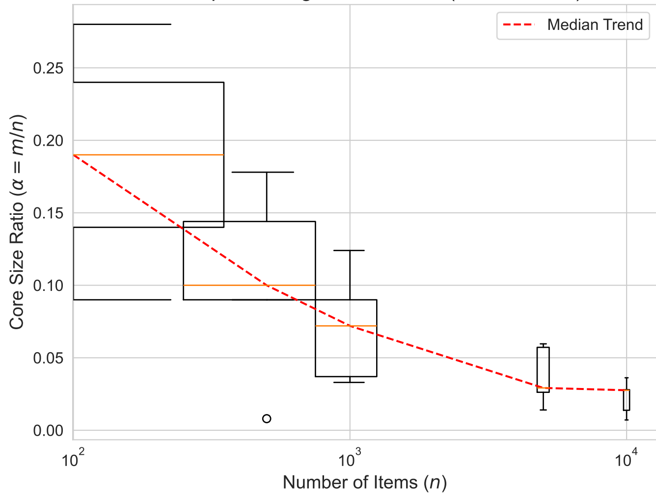
LP Preprocessing Effectiveness (Uncorrelated)
