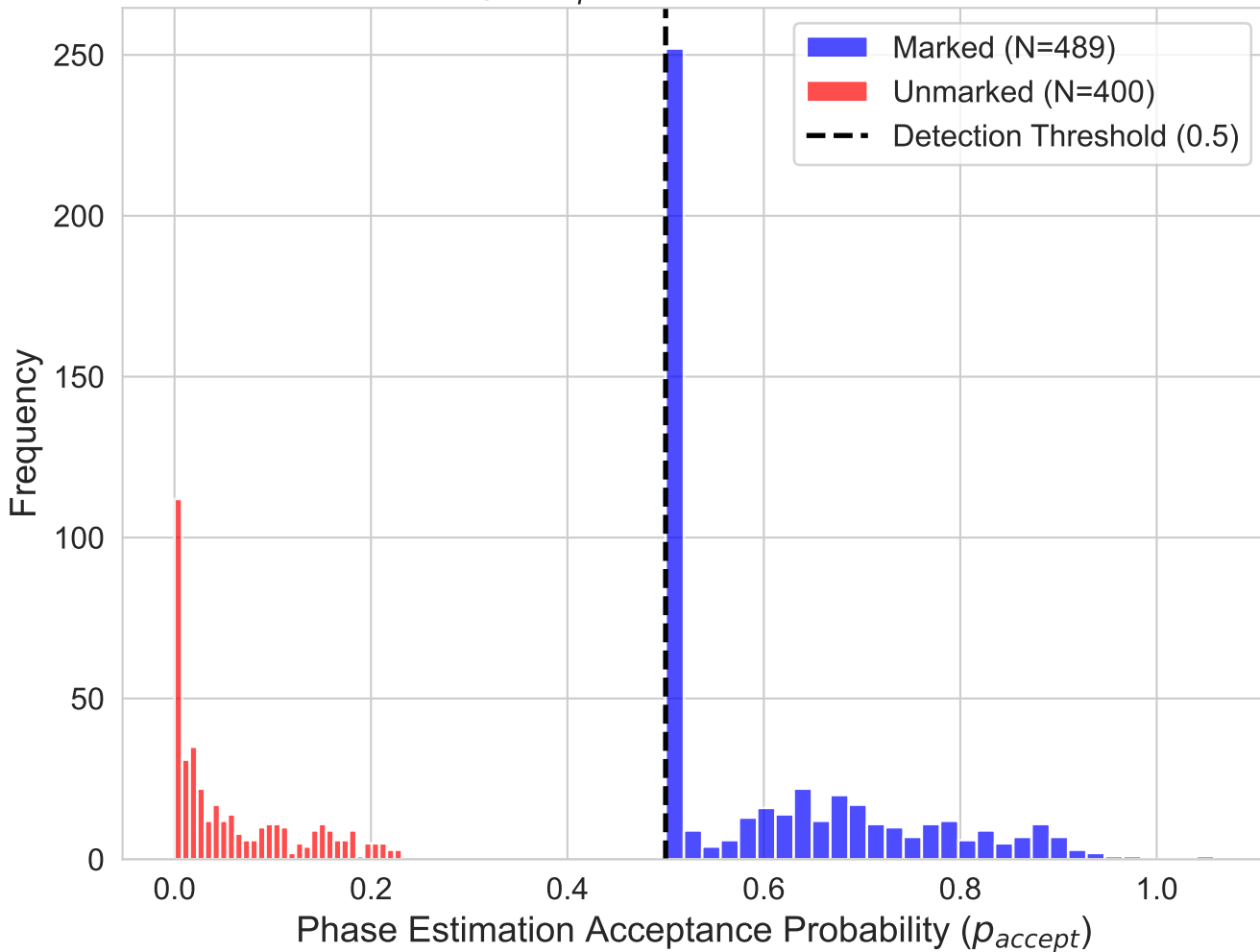
Distribution of p_{accept} for Simulated Quantum Walks
