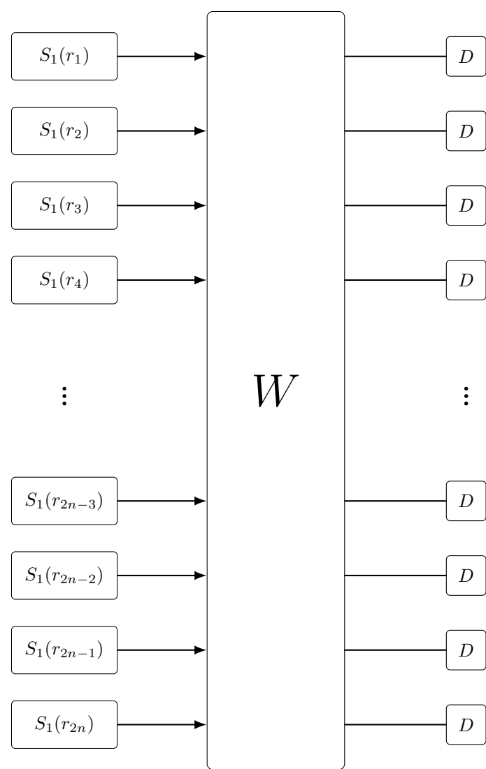
(a) Standard GBS
