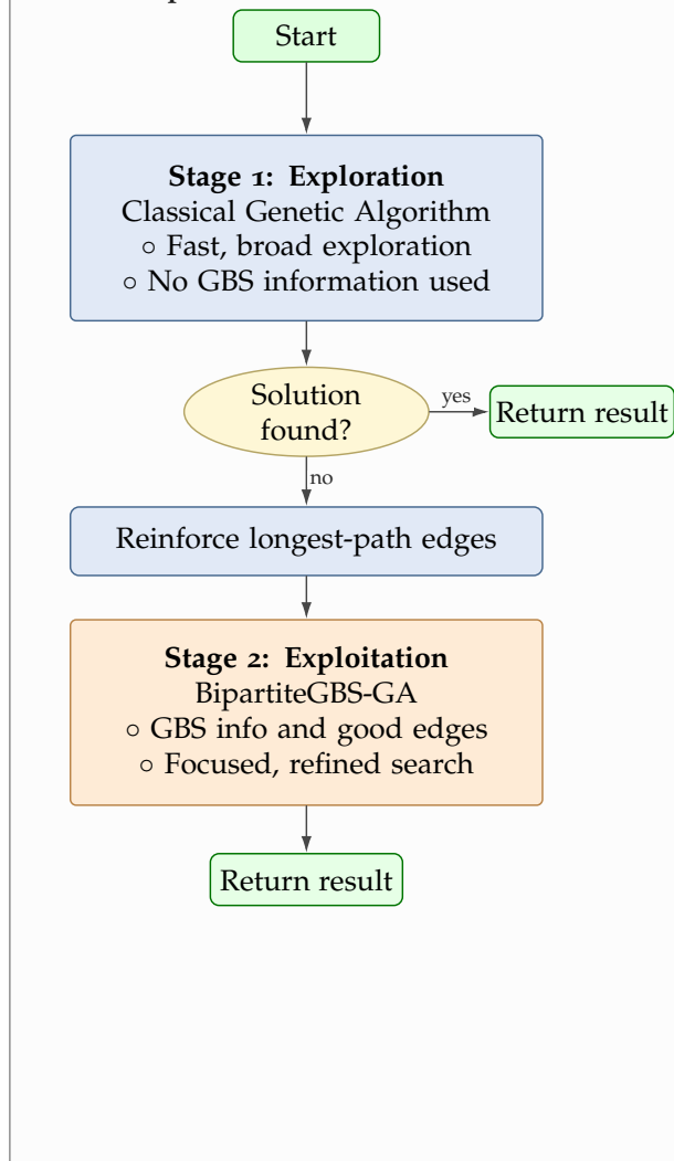
(c) MS-BipartiteGBS-GA
