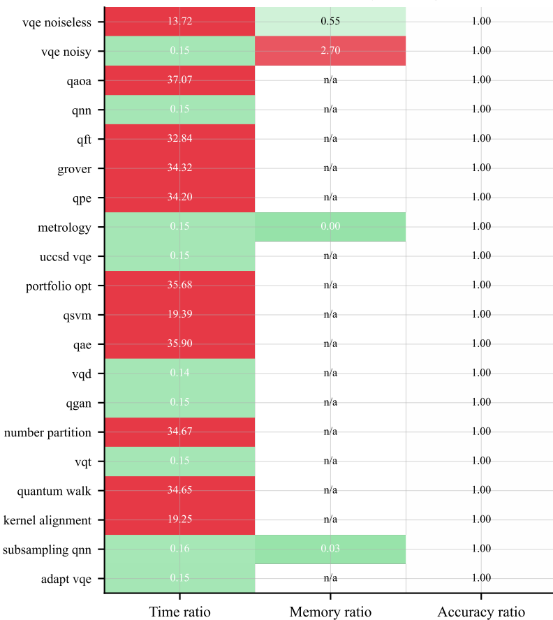
LRET Performance Summary (20 Algorithms)
