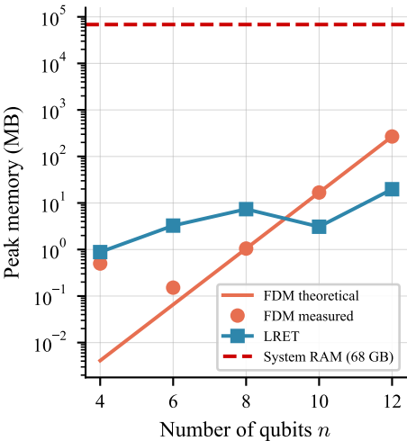
(a) Memory Scaling
