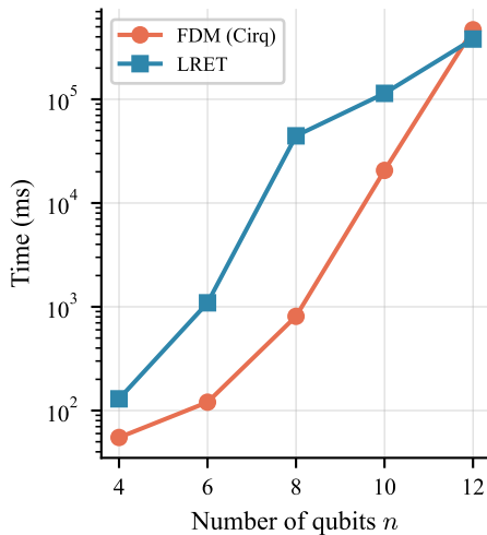
(b) Time Scaling
