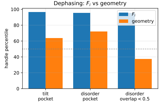
FIG. 3. Dephasing handle percentile, F_i vs geometry, in the pocket and (disorder) where the two selectors most disagree. F_i wins; geometry collapses below the median at low overlap.
