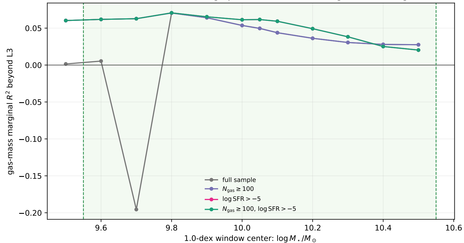
CAMELS-TNG CV: lower-edge persistence after catalog-floor cleaning
