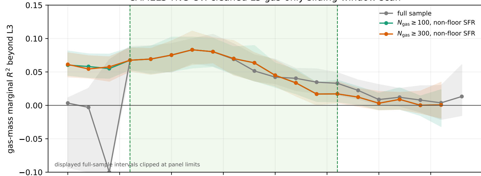
CAMELS-TNG CV: cleaned L3 gas-only sliding-window scan
