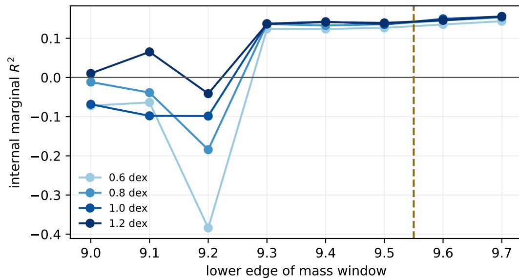
CAMELS-TNG CV: diagnostics of the lower intermediate-mass boundary
