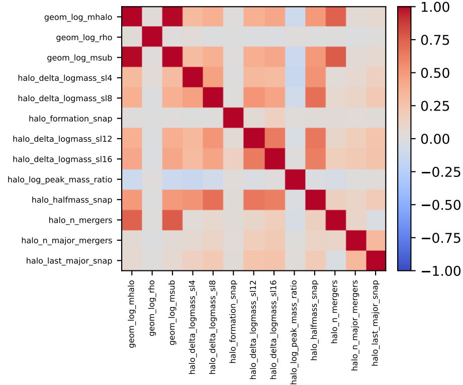
L3 feature correlation matrix
