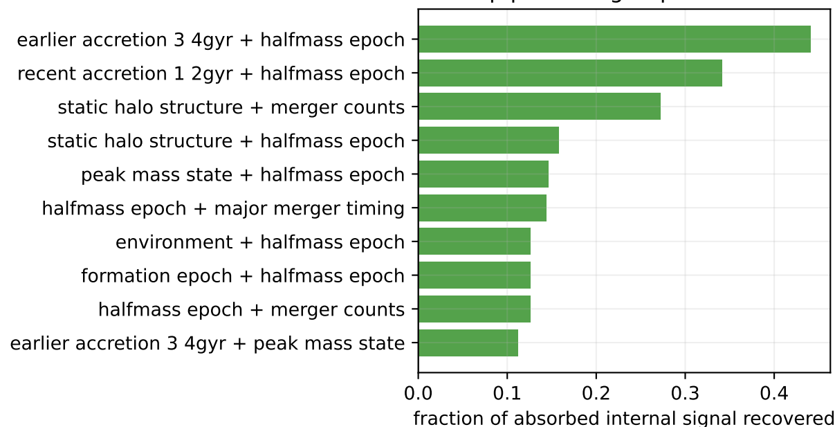
Correlated L3 assembly manifold
