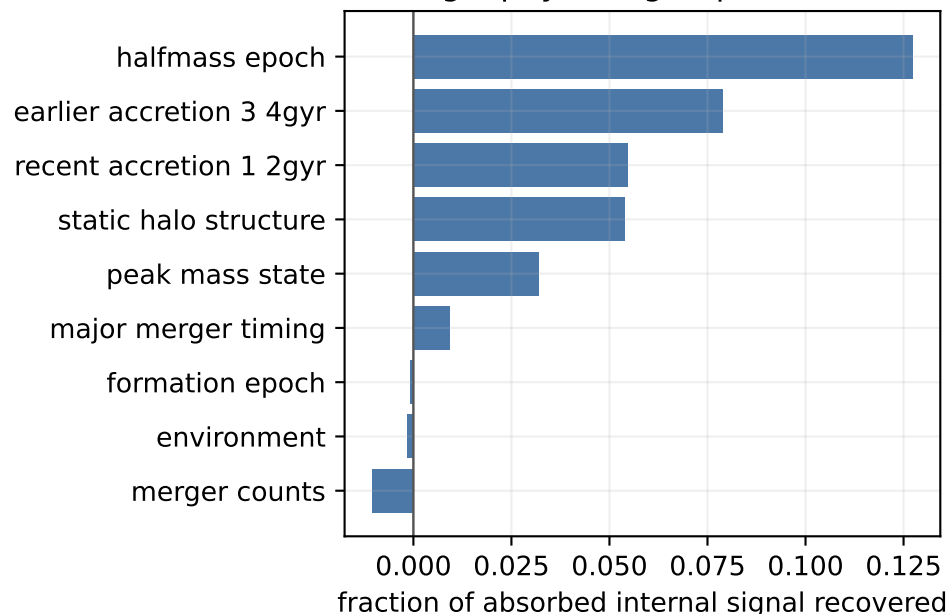
Top pairwise group removals
