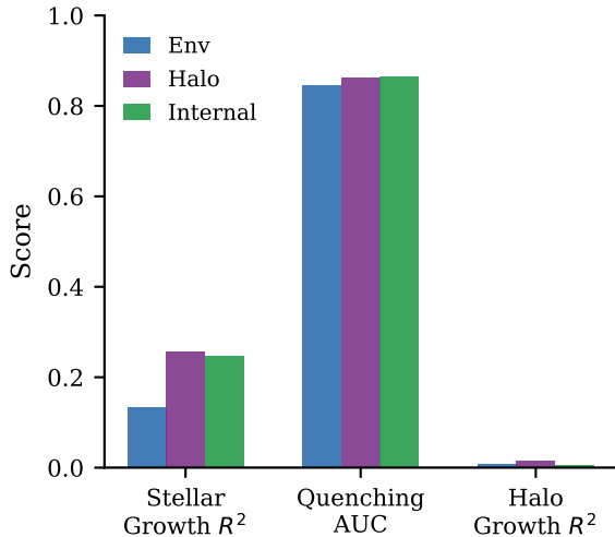
TNG SubLink
