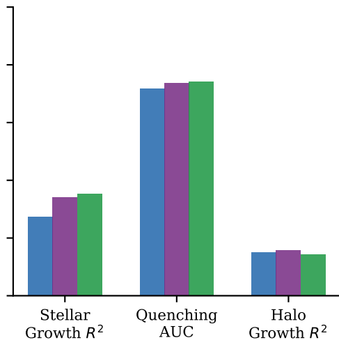
SIMBA Spatial
