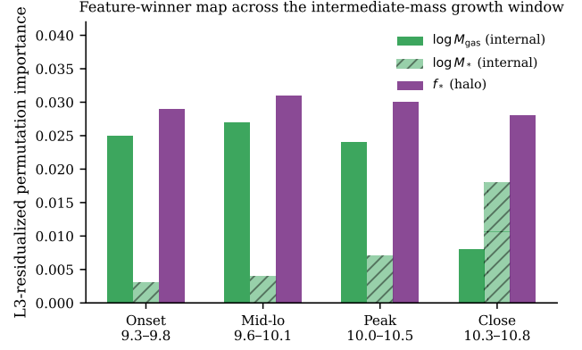
Figure 4. Feature-winner map across the intermediate-mass growth regime. L3-residualized permutation importance at four window positions. Gas mass (dark green) dominates the internal class at onset through peak; stellar mass (hatched) is the sole surviving internal feature at the close. f_* (purple) is the stable halo carrier throughout.
