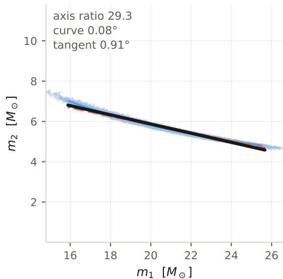
clean success (high elongation) GW241011_233834 (O4b)
