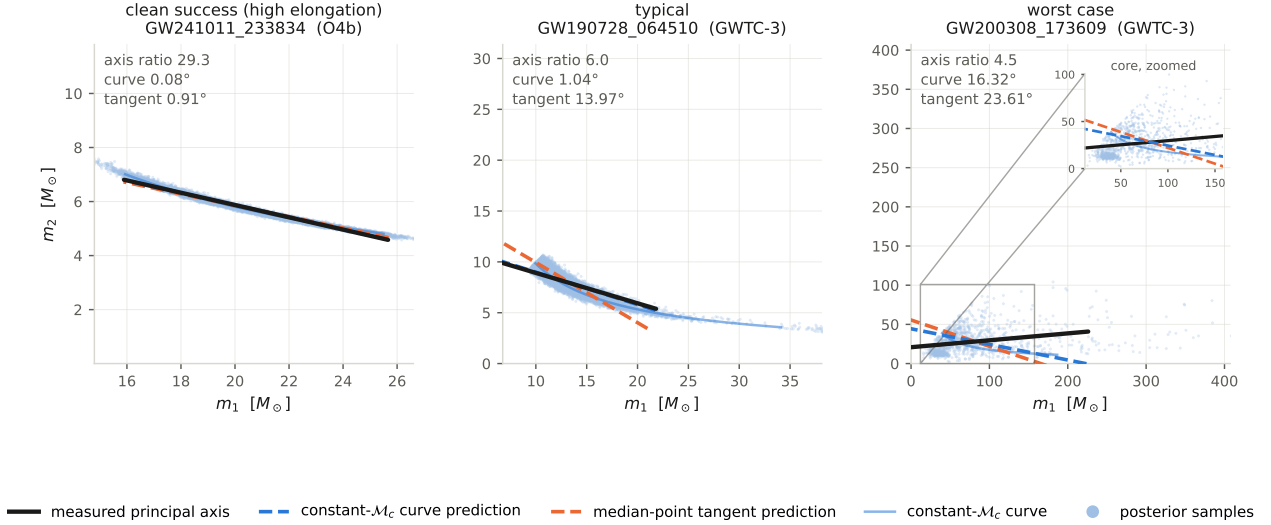
Figure 3: Posterior geometry for three events chosen by fixed rules — clean success ( high elongation ) GW241011.233834 (O4b, axr 29.3, curve 0.08^\circ , tangent 0.91^\circ ); typical GW190728_064510 (GWTC-3, axr 6.0, curve 1.04^\circ , tangent 13.97^\circ ); worst case GW200308_173609 (GWTC-3, axr 4.5, curve 16.32^\circ , tangent 23.61^\circ ). Each panel shows the posterior samples, the constant- \mathcal{M}_c curve, the measured principal axis and the two predicted orientations, on equal-aspect axes. The worst case is included by rule rather than chosen, and carries a zoom inset on its dense core; its failure is genuine, the error remaining at 16.2\text{--}17.5^\circ when the sample is trimmed to its central 90%. Across all elongated events the tangent beats the curve for 15% of events, rising to 31% above \text{axr} = 8 .
