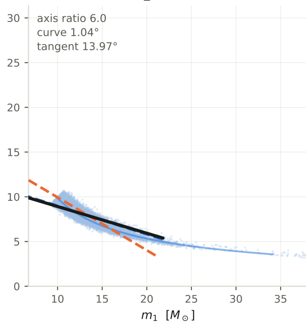
typical GW190728_064510 (GWTC-3)
