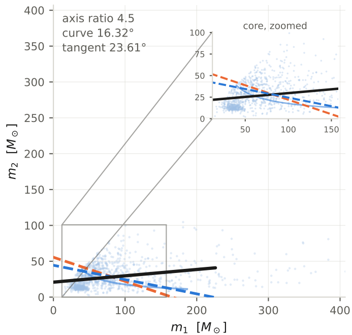
worst case GW200308_173609 (GWTC-3)
