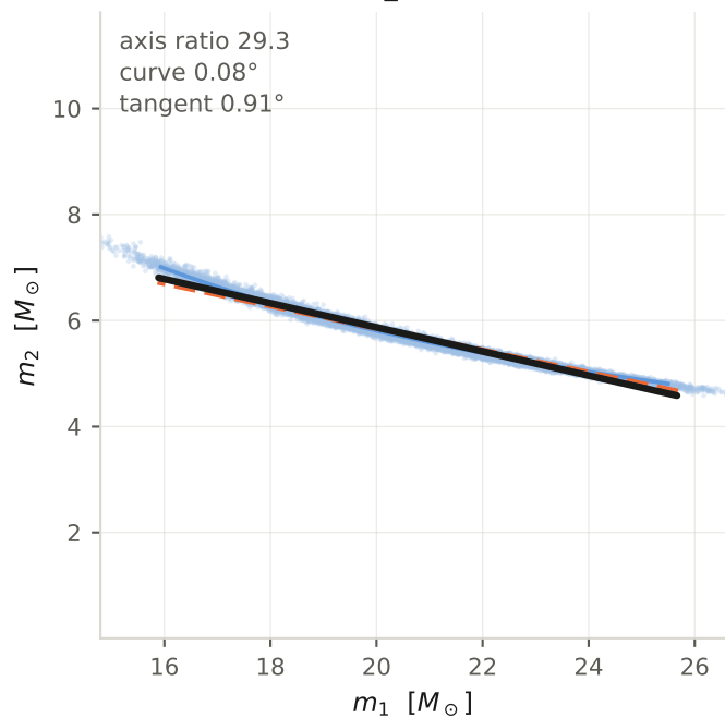
clean success (high elongation) GW241011_233834 (O4b)
