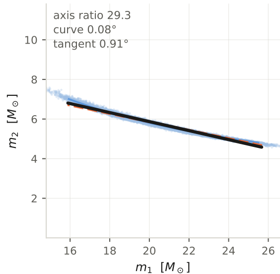
clean success (high elongation) GW241011_233834 (O4b)
