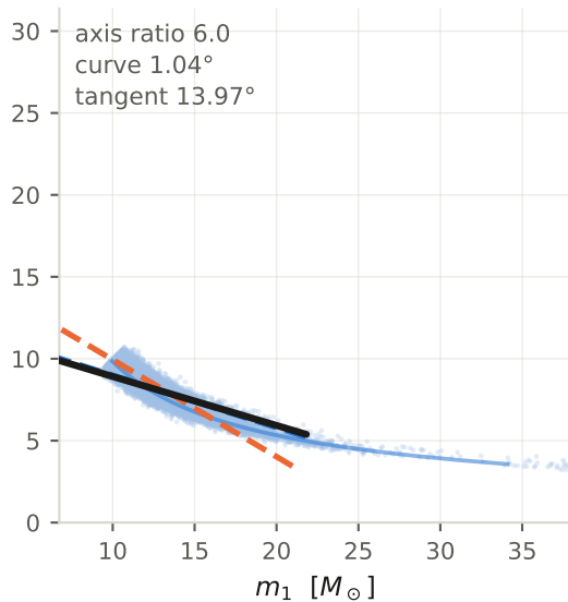
typical GW190728_064510 (GWTC-3)
