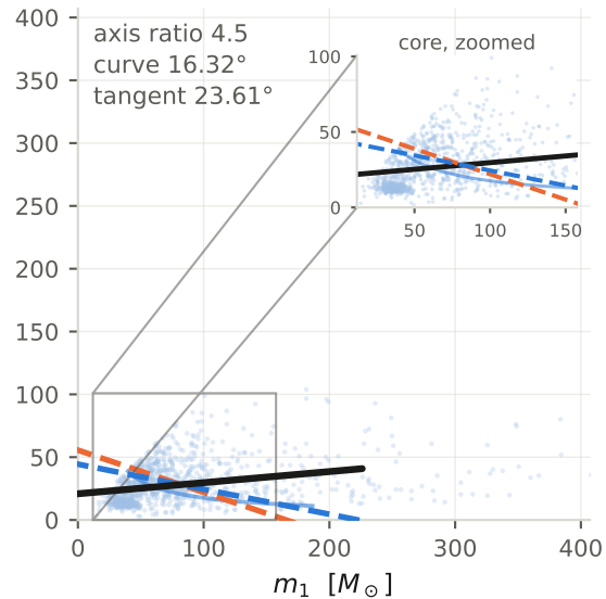
worst case GW200308_173609 (GWTC-3)
