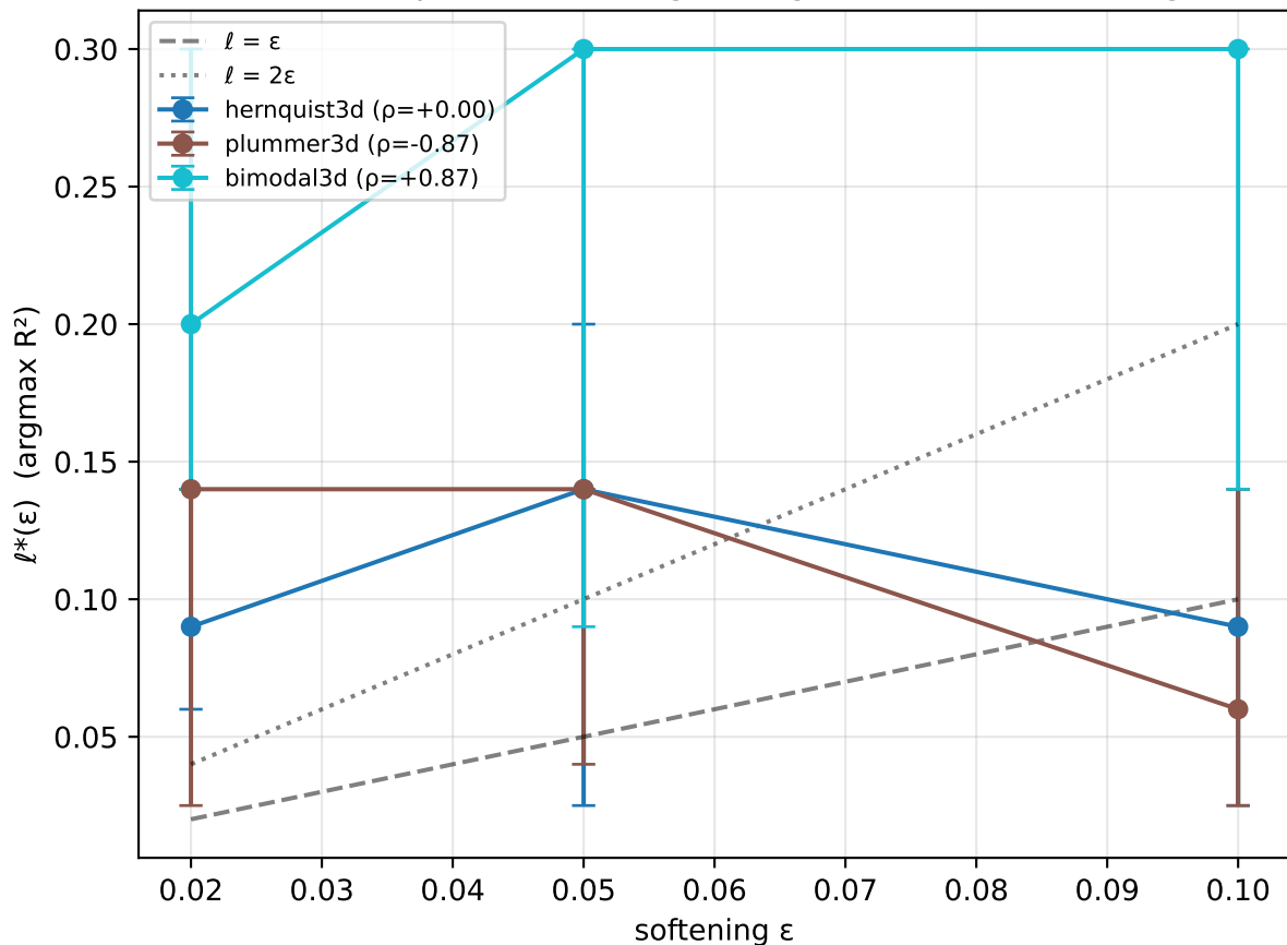
Does the optimal coarse-graining scale track softening?
