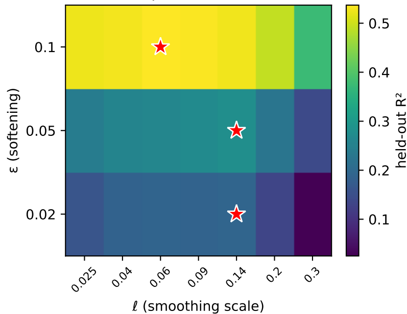
plummer3d
