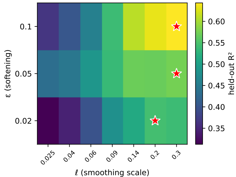
bimodal3d
