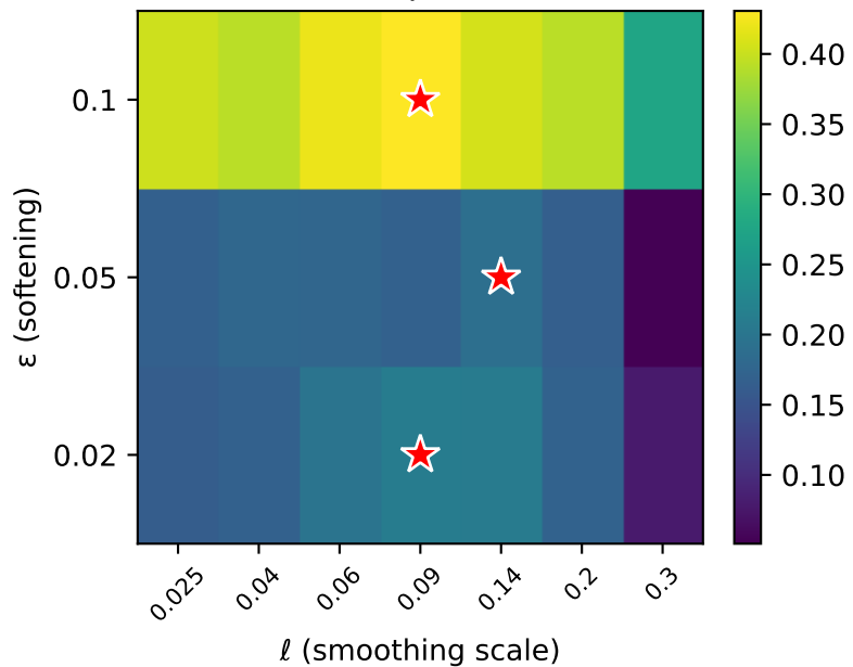
hernquist3d
