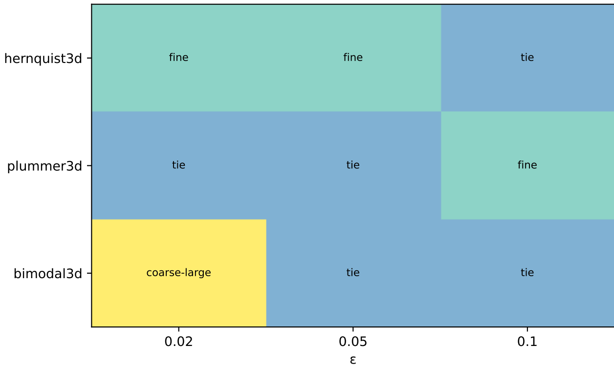
Winner map (description that best predicts \Delta C8 -early)
