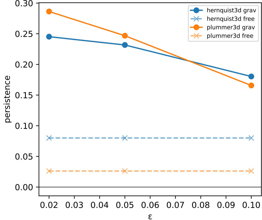
Persistence: gravity vs free-streaming
