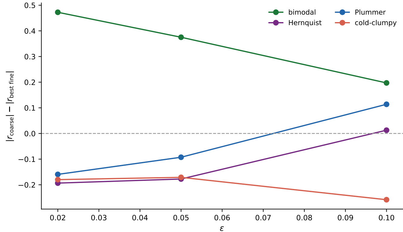
Coarse advantage vs softening ( N = 1024 , direct-isolated)
