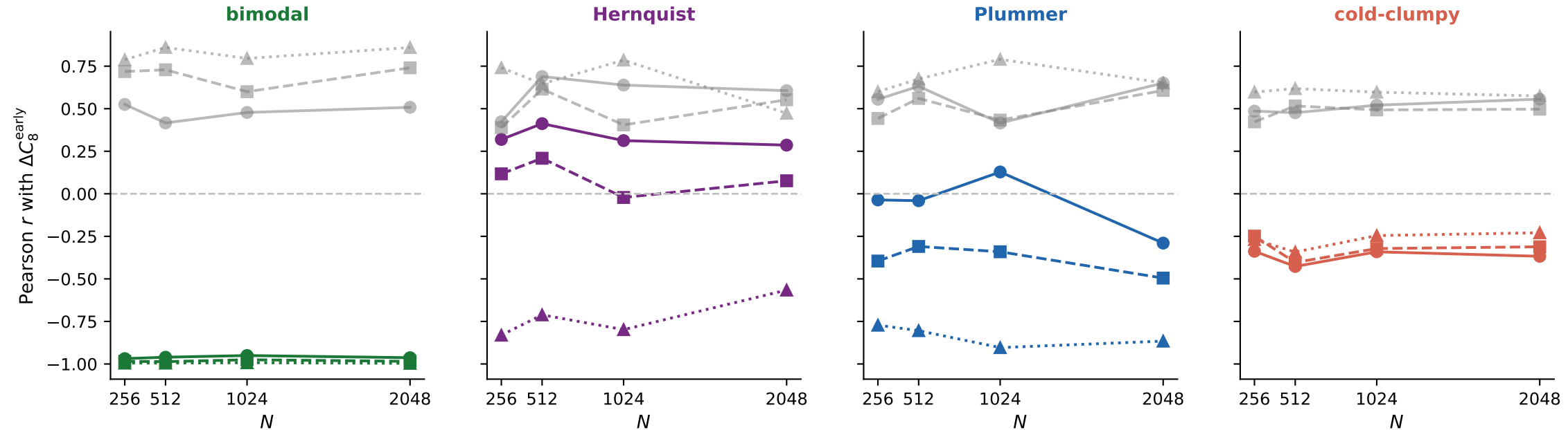
N-scaling: coarse predictor vs best fine predictor (direct-isolated)
