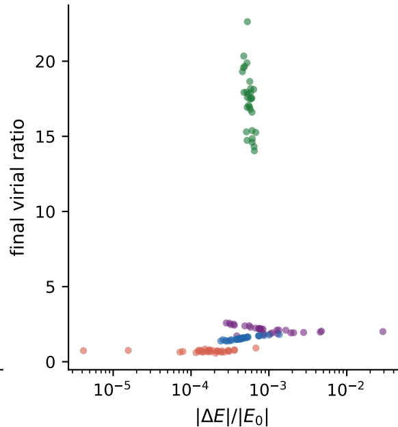
Energy drift vs final virial ratio
