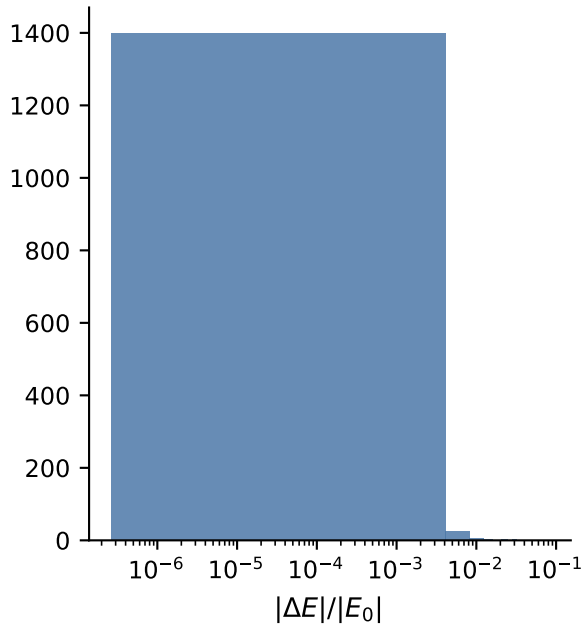
Relative energy drift
