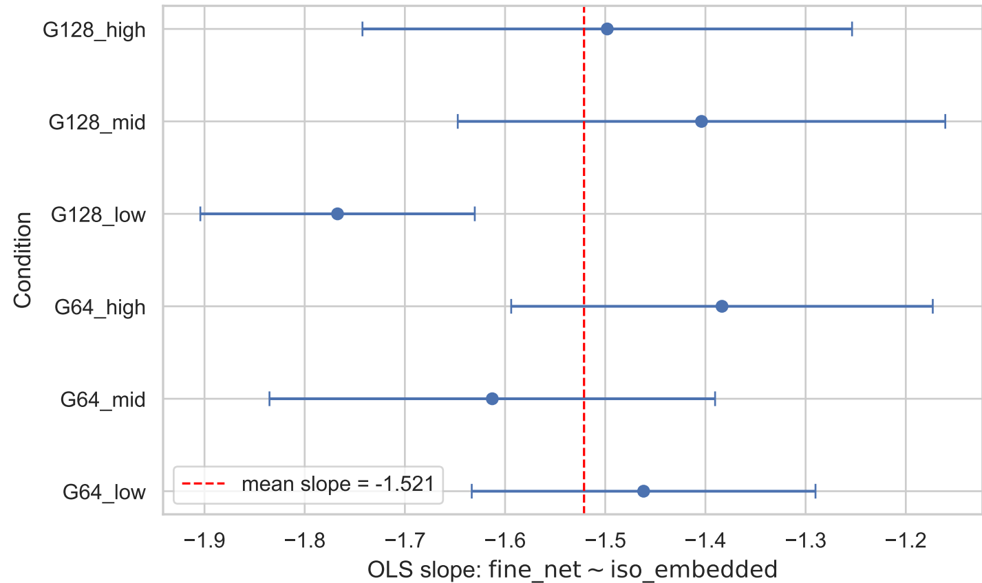
Study D — slope summary, CV = 0.087
