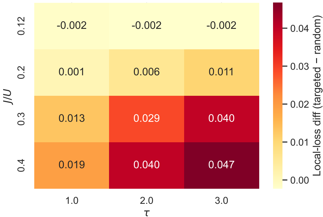
Local-loss difference across regimes ( L = 6 )
