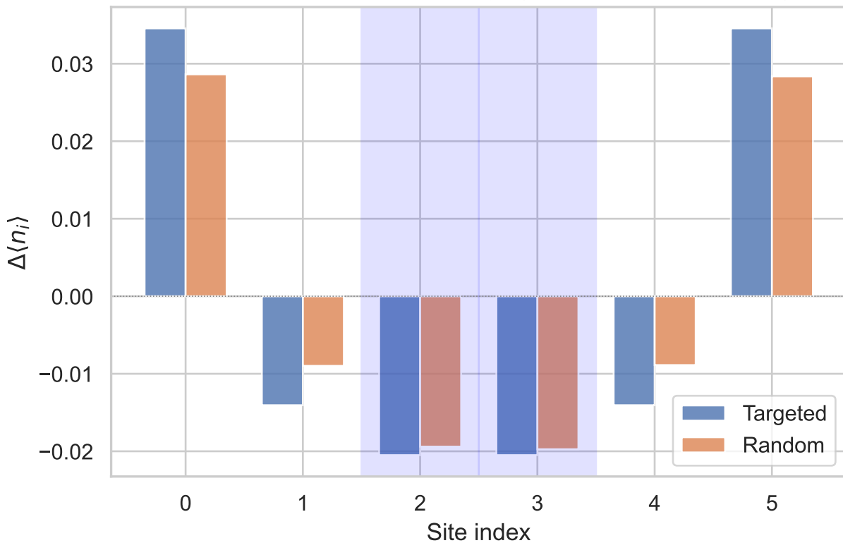
Site-resolved occupation change ( J/U = 0.30 , L = 6 , \tau = 2 )
