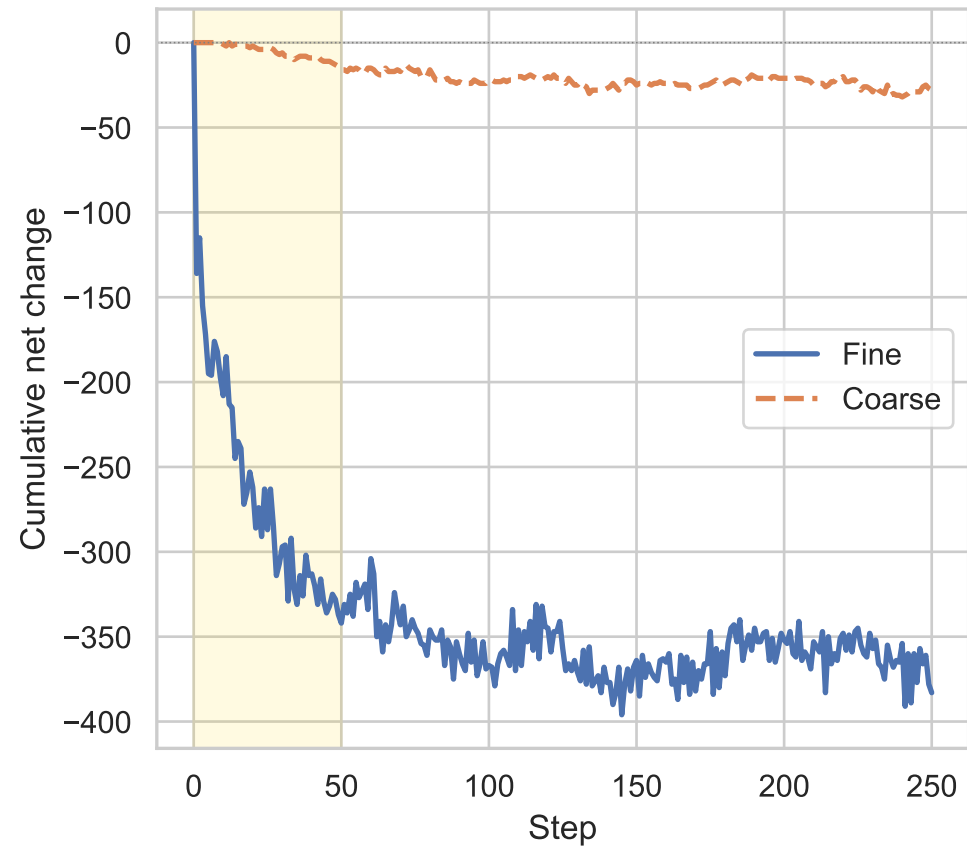
G > 0 , world 687, G = 0.621
