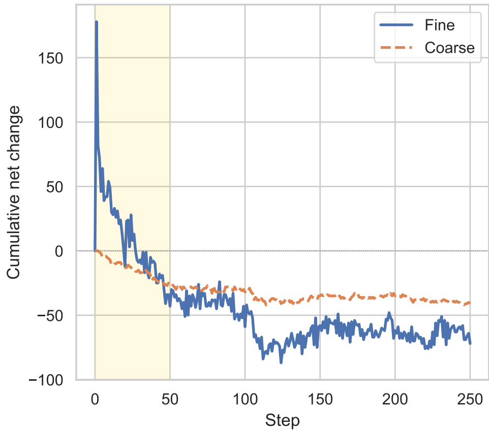
G < 0 , world 765, G = -0.321
