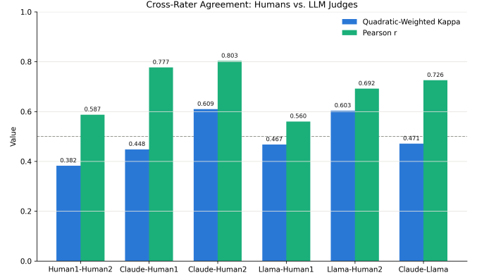
Fig. 2. Cross-rater agreement (quadratic-weighted Cohen’s \kappa and Pearson r ) across all six rater pairs: two human annotators, the original Claude judge, and a second LLM (Llama-3.3-70B). All comparisons, including the Human1–Human2 baseline, fall within a similar range, indicating the categorical noise observed throughout the validation is inherent to the evasion construct itself rather than specific to any single rater.
