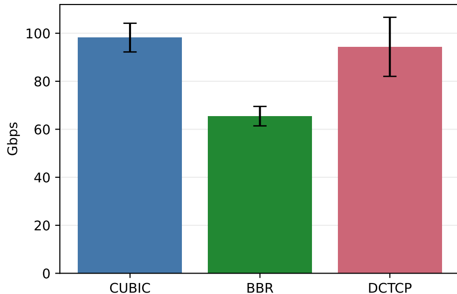
Receiving throughput
